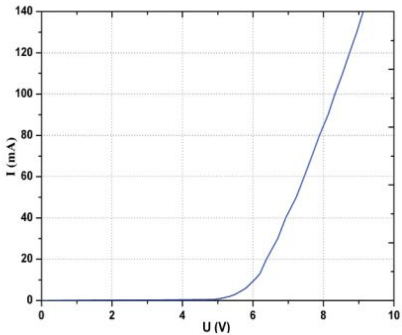
I-V characteristic
